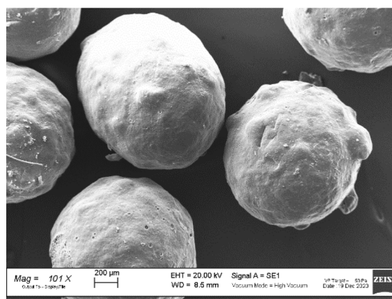
Fig. 3. SEM photomicrographs of units cushion-coated with PEG1500 to 50 % weight gain. (uGIC 50 ).
