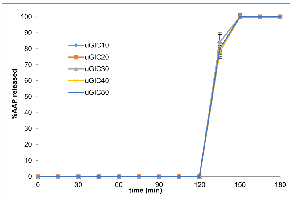
Fig. 4. Release profiles of AAP from individual gastro-resistant units cushion-coated with PEG1500 to 10–50% weight gain.
