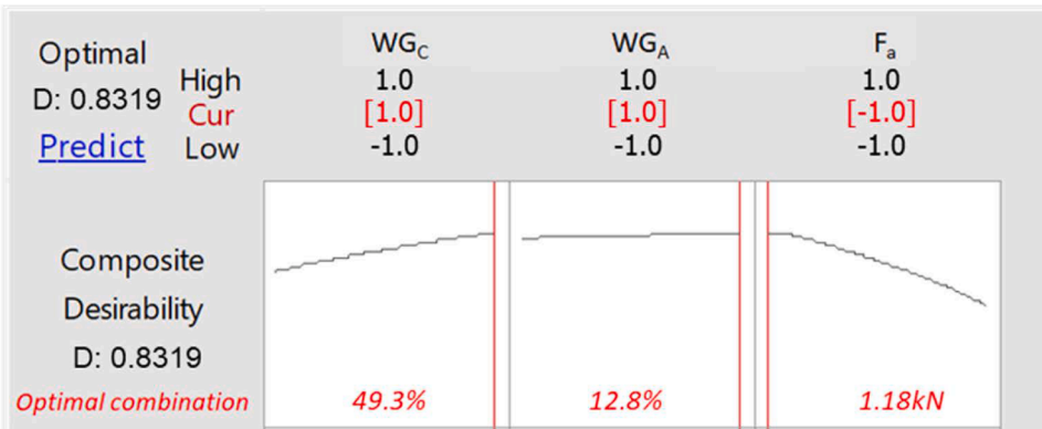
Fig. 8. Trend of the composite desirability function and optimized conditions for manufacturing of tableted MUPSSs.
